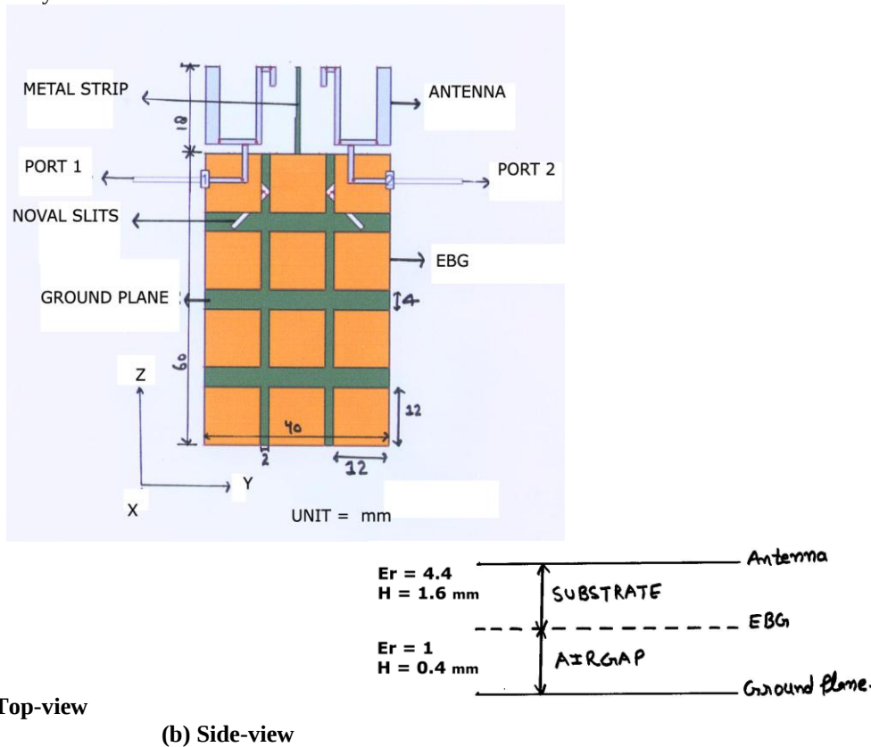
Fig 1: MIMO Antenna with EBG structure.
