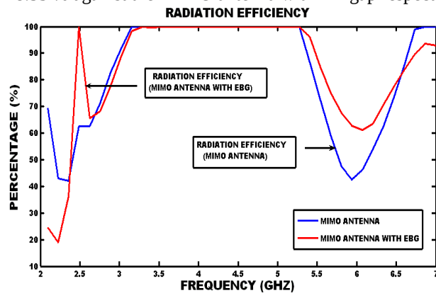
Fig 5(b) Radiation Efficiency vs. Frequency
