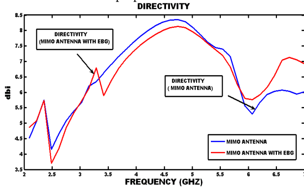
Fig 3: Directivity vs. Frequency
