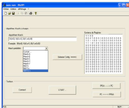
Fig. 2 : User interface
