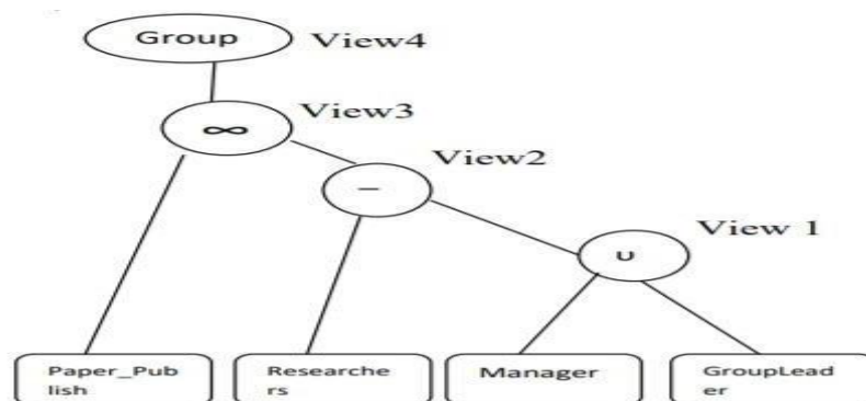
Figure 1: Expression tree
