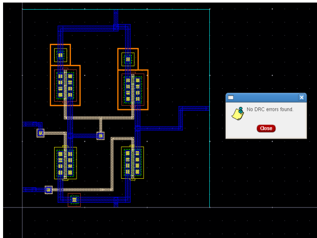
Fig 10: Layout of Comparator with Assura DRC
