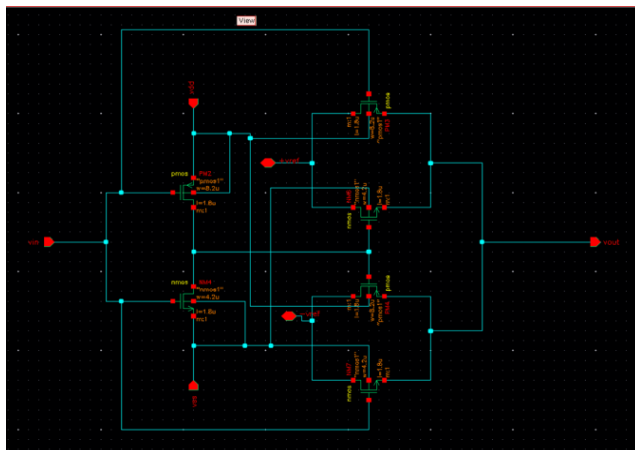
Fig 11: Schematic view of DAC
