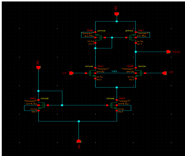
Fig 3: schematic view of differential amplifier
