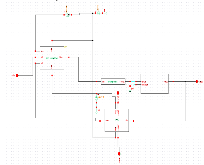
Fig 2: Complete 1-bit sigma delta modulator schematic design
