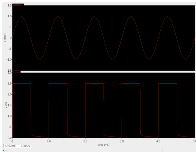
Fig 13: 1- Bit Sigma delta output
