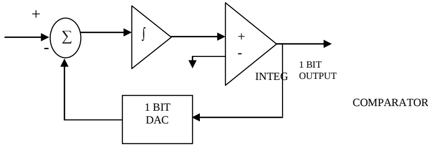
Fig 1: 1 bit Sigma-delta Modulator
