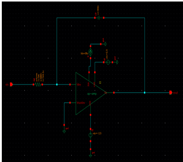
Fig 7: Schematic view of Integrator
