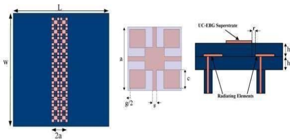
Figure 2: Narrowband isolation is achieved using an antenna array with EBG
