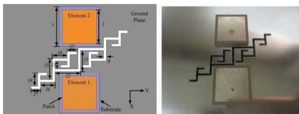
Figure 1: An isolation solution for narrowband applications using FDGS antennas in a close-packed configuration:
