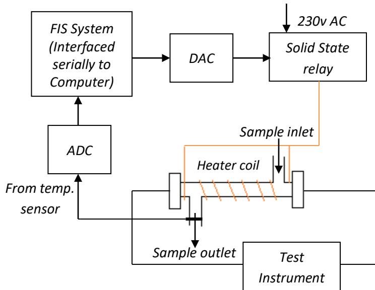
Figure 2: Block diagram of Experimental Setup
