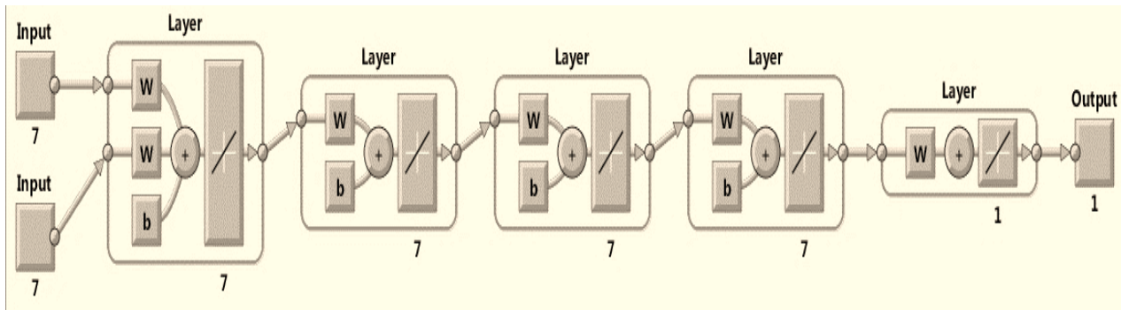
Fig. 2: Custom designed Back Propagation Neural Network (BPNN) model for STLP for SPDCL of A.P.
