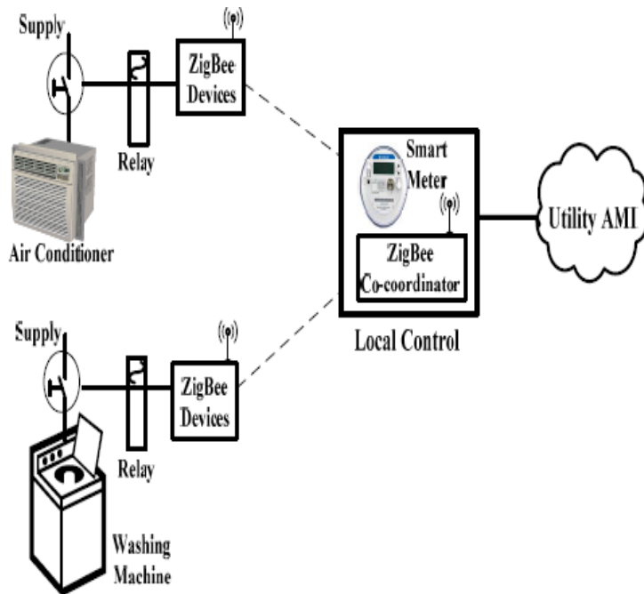
Fig. 6 ZigBee technology for smart home area network.
